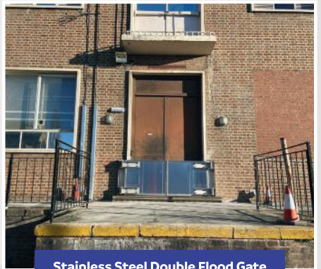
Stainless Steel Double Flood Gate
